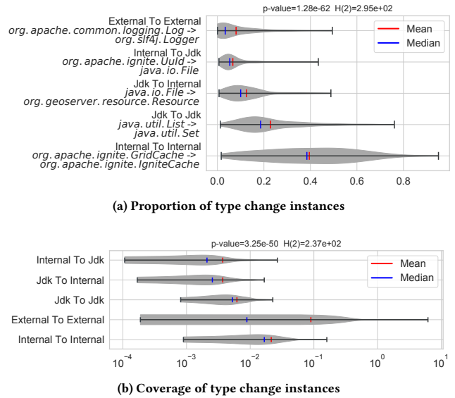
Figure 4: Project-level distribution per namespace kind
