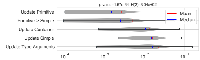
(b) Coverage of type change instances
