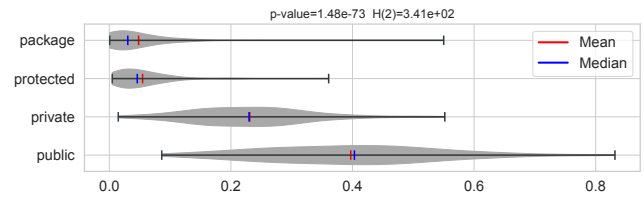
(a) Proportion of type change instances
