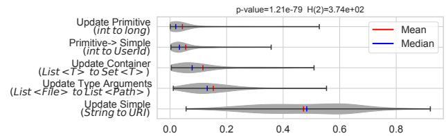
(a) Proportion of type change instances
