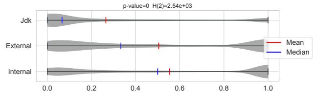
Figure 6: Project-level distribution of type change coverage
