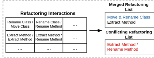
Fig. 2: An overview of RefMerge’s merging algorithm
